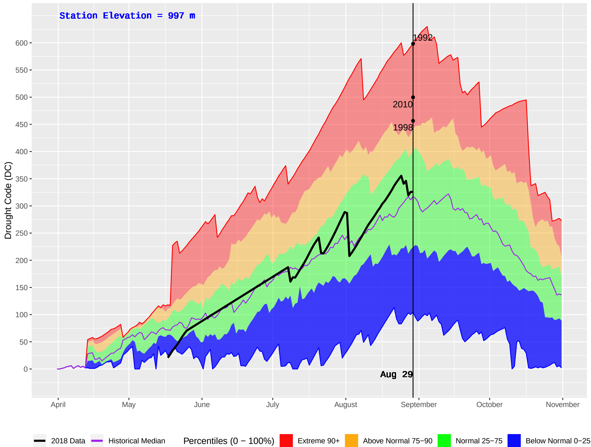
JERRY (190) : Historical (1988–2016) and Current (2018) Daily Drought Code (DC)
