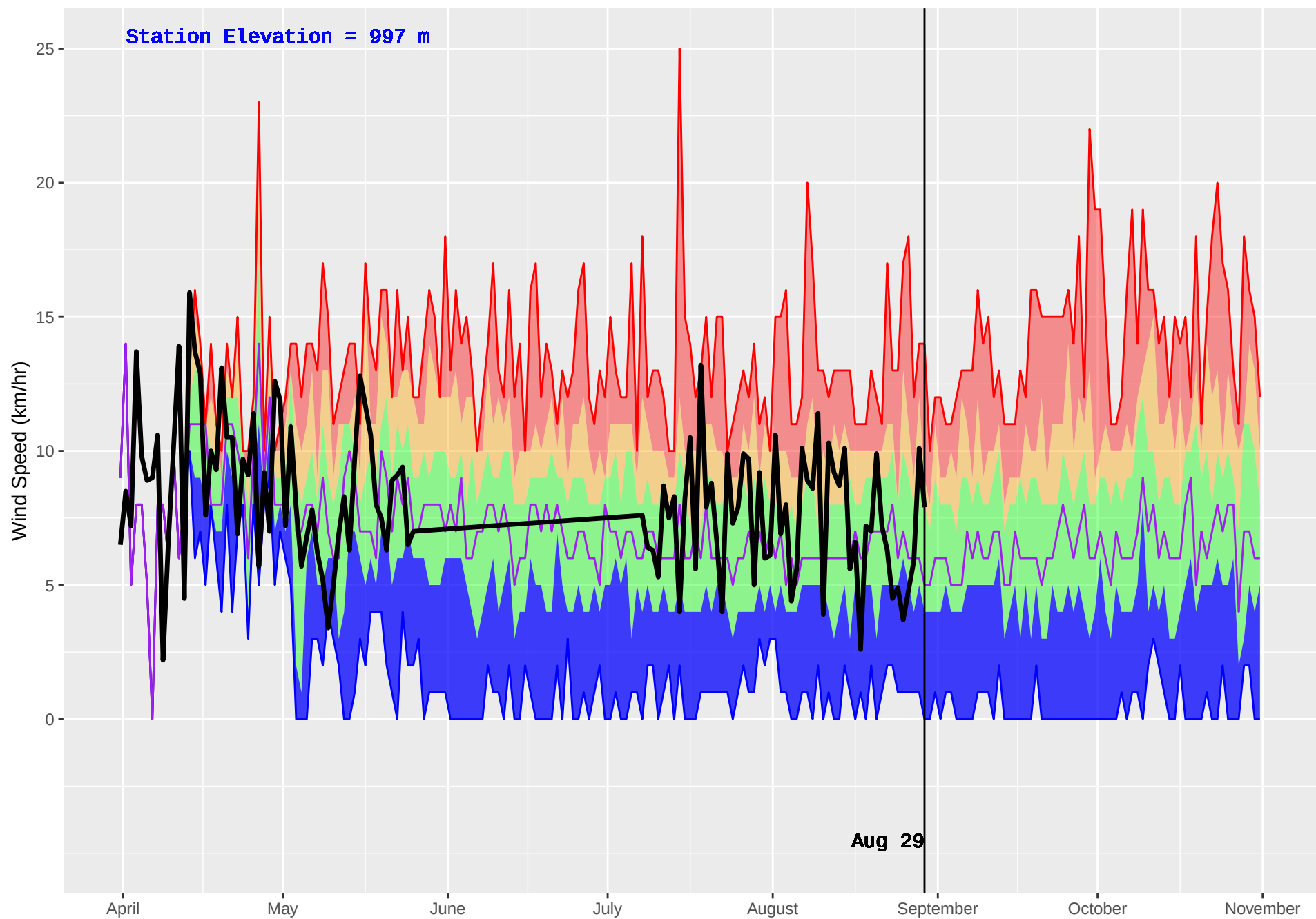
JERRY (190) : Historical (1988–2016) and Current (2018) Daily Wind Speed
