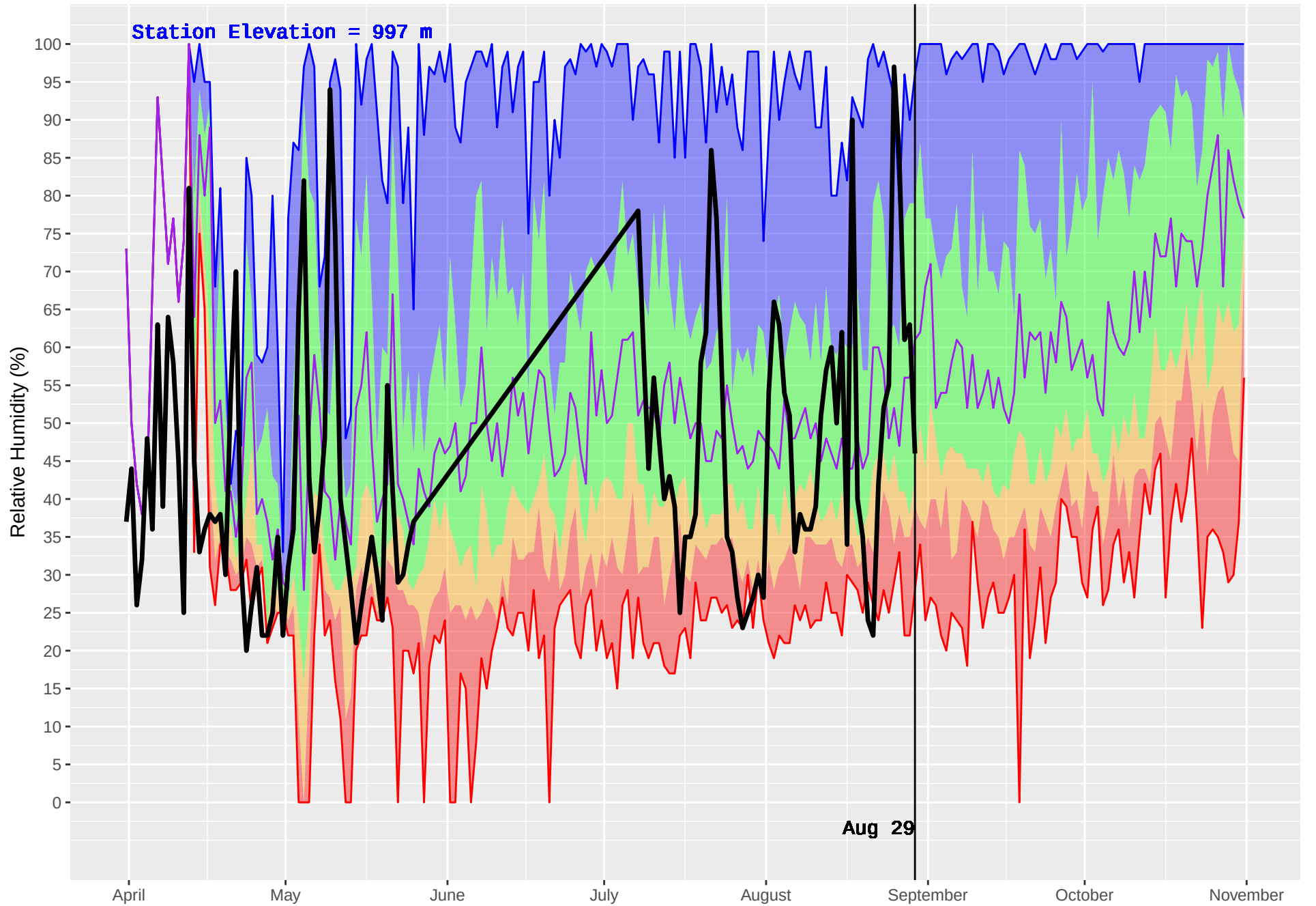
JERRY (190) : Historical (1988–2016) and Current (2018) Daily Relative Humidity
