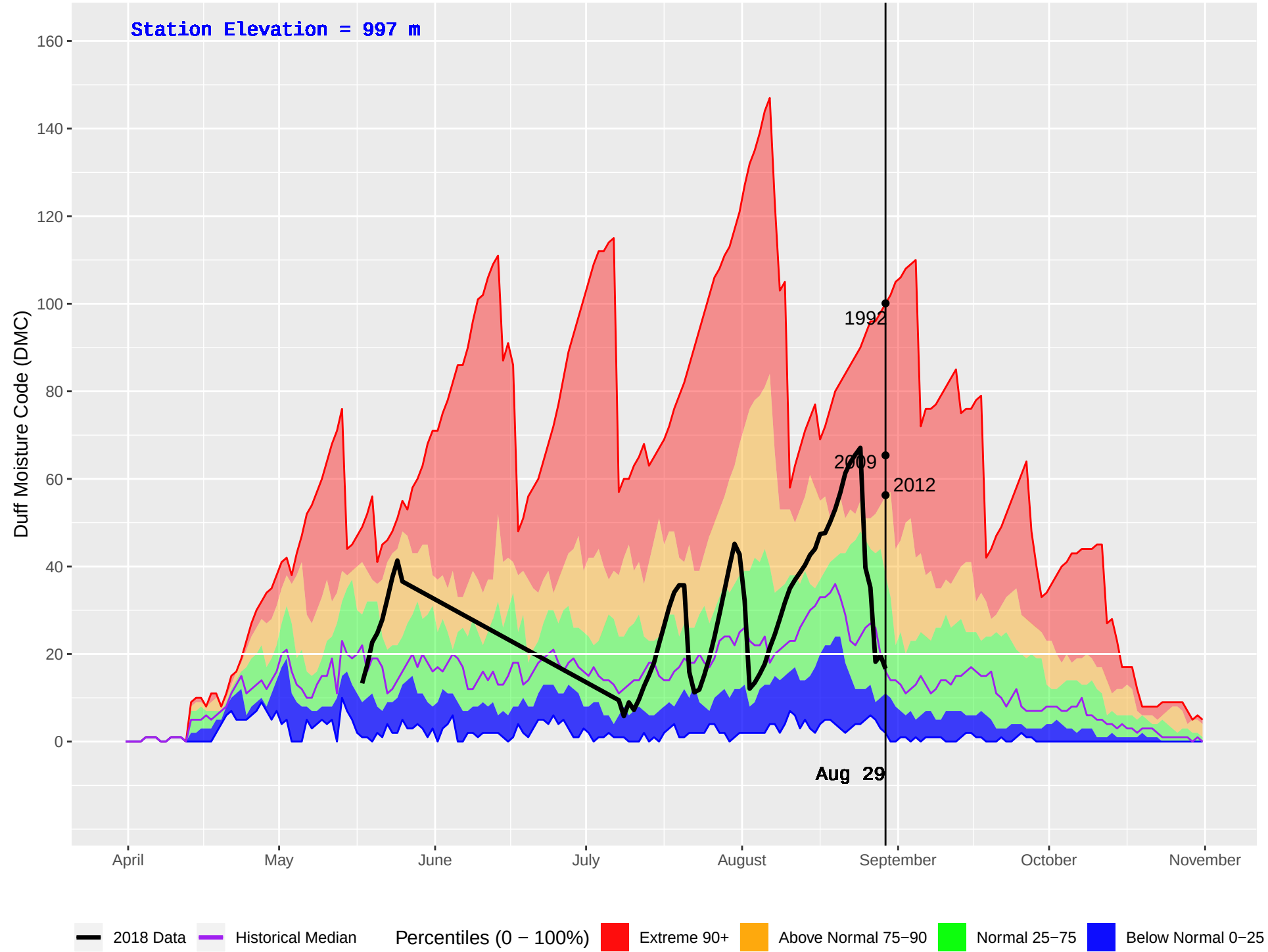
JERRY (190) : Historical (1988–2016) and Current (2018) Daily Duff Moisture Code (DMC)
