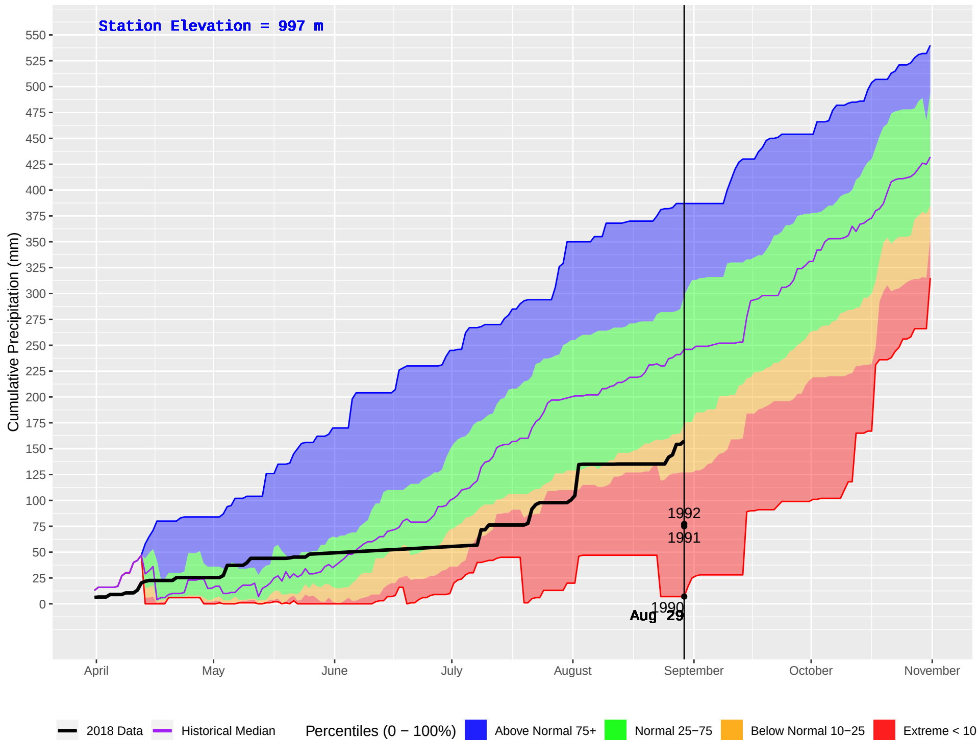
JERRY (190) : Historical (1988–2016) and Current (2018) Daily Cumulative Precipitation
